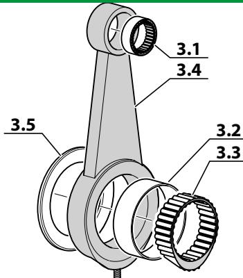
KIT 1a - 13-00-0050/R KIT 1b - 13-00-0050/TR/R
