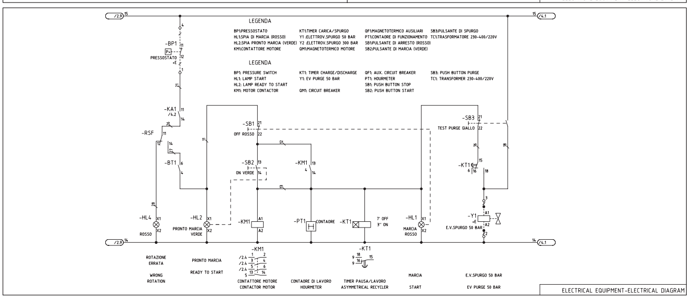
ELECTRICAL EQUIPMENT-ELECTRICAL DIAGRAM
