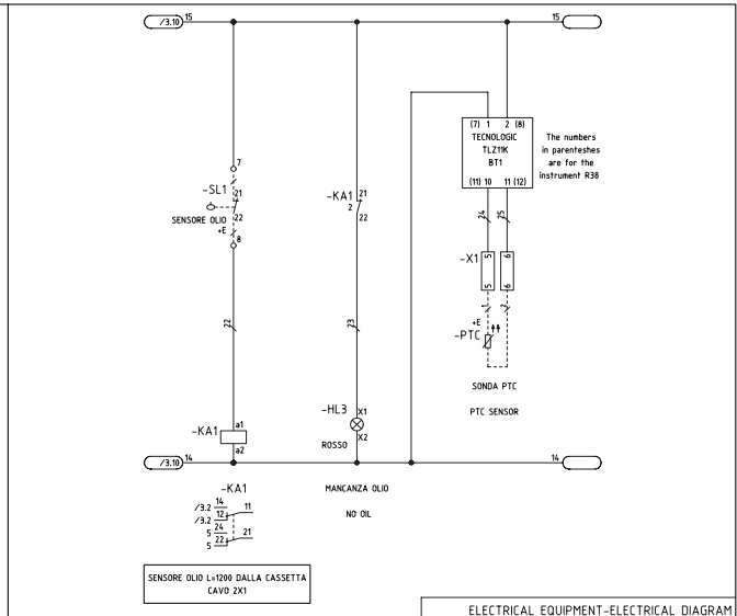
ELECTRICAL EQUIPMENT-ELECTRICAL DIAGRAM
